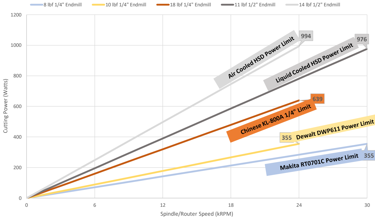
Cutting Power (Watts) and Force (lbf) vs. Spindle/Router Speed (kRPM) and Endmill Diameter (in) (Note that Material Removal Rate (MRR - in 3 /minute) is Proportional to Cutting Power)
