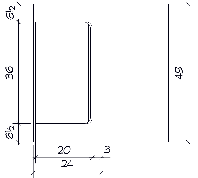
XXL SHAPOKO Enclosure .75" Plywood
